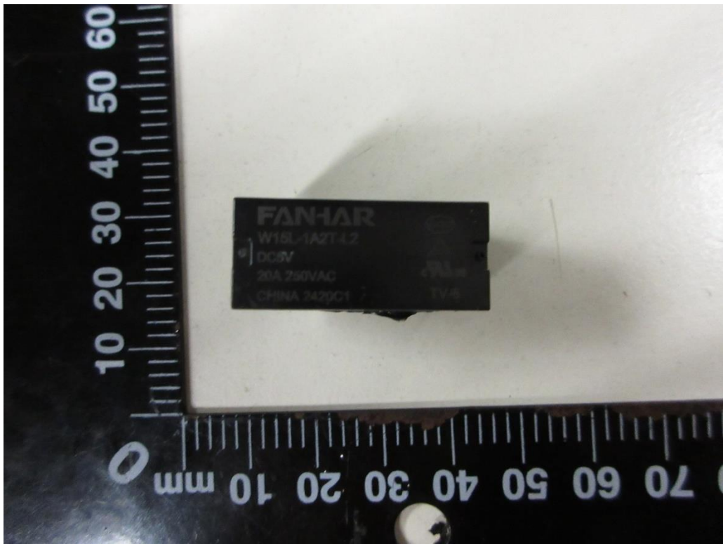
Relay (W15L-1A2T-L2-DC5V)
