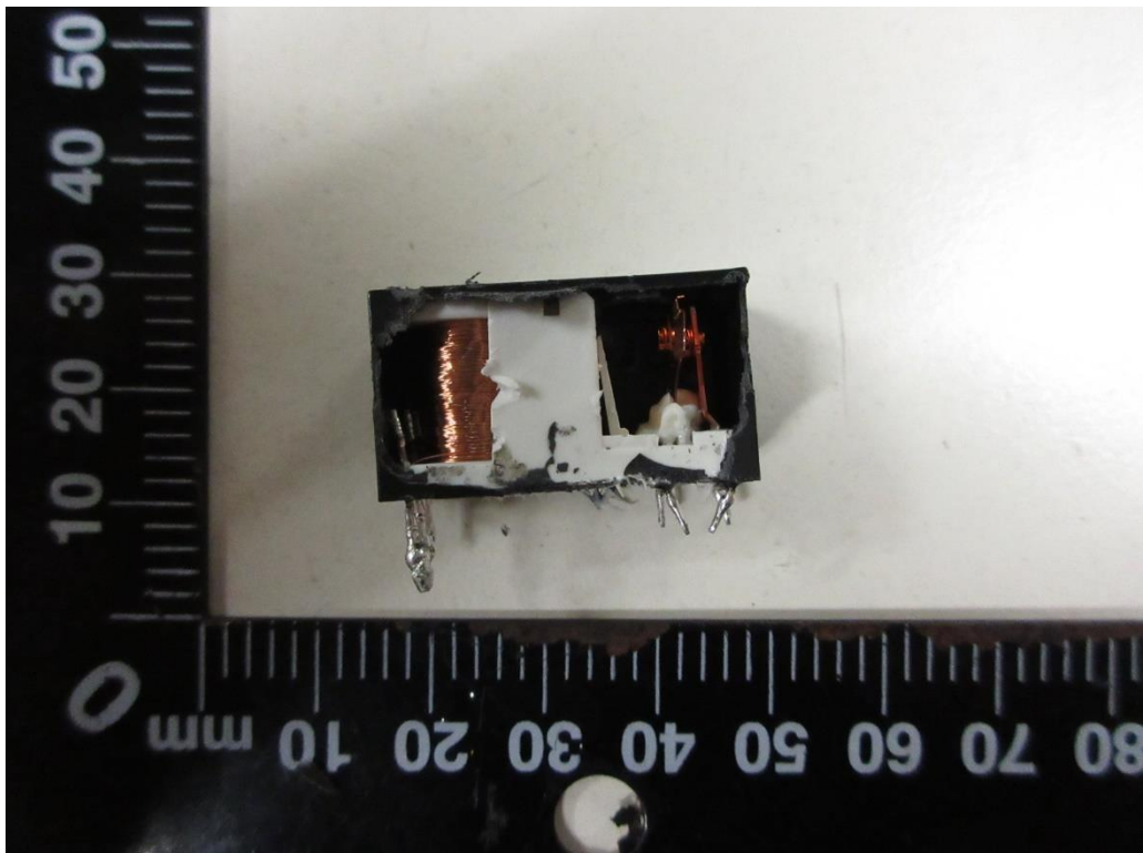
Relay (W15L-1A2T-L2-DC5V)
