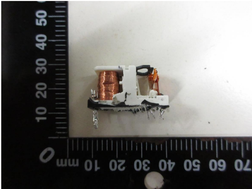
Relay(W15L-1A2T-L2-DC5V)
