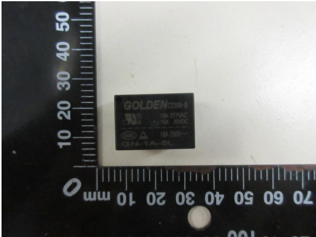
Relay (GN-1A-5L)
