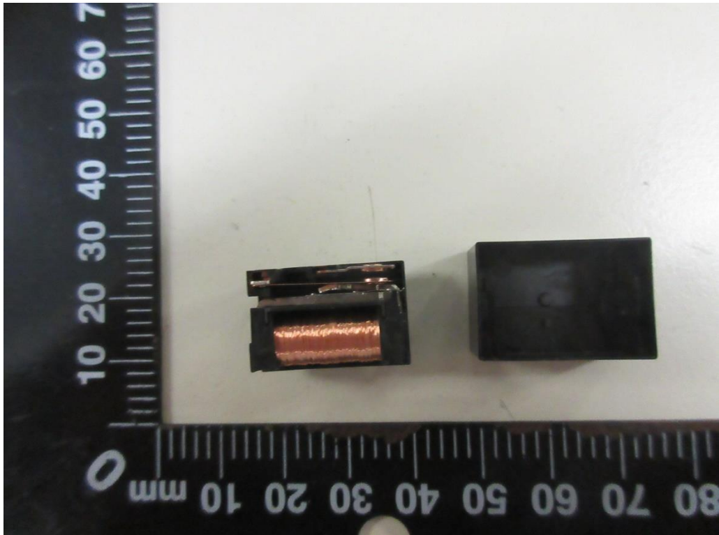
Relay (GN-1A-5L)
